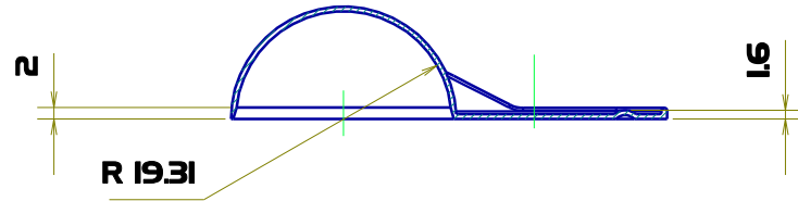
Sect. A-A
