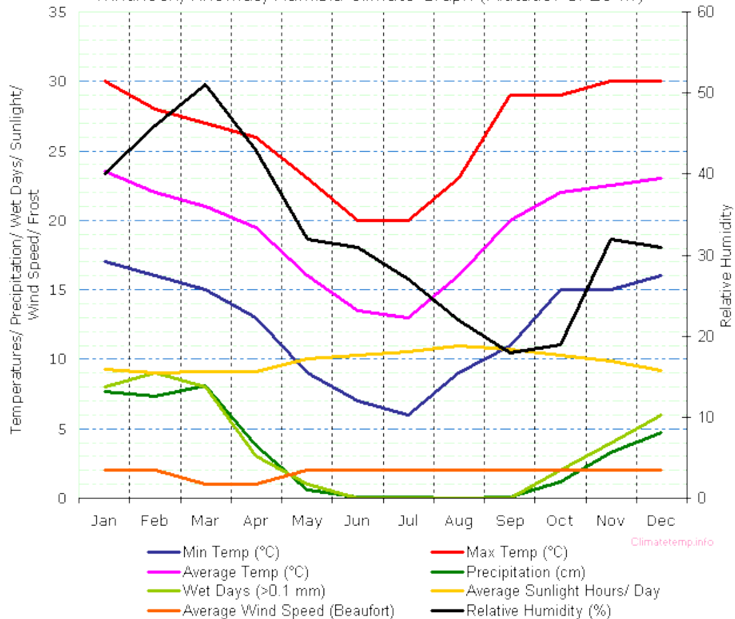
Windhoek, Khomas, Namibia Climate Graph (Altitude: 1728 m)
