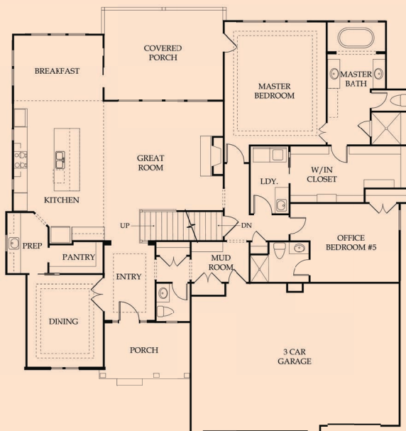
MAIN LEVEL 2,308 SQFT
