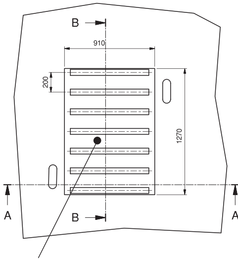
cavo - Excavation
