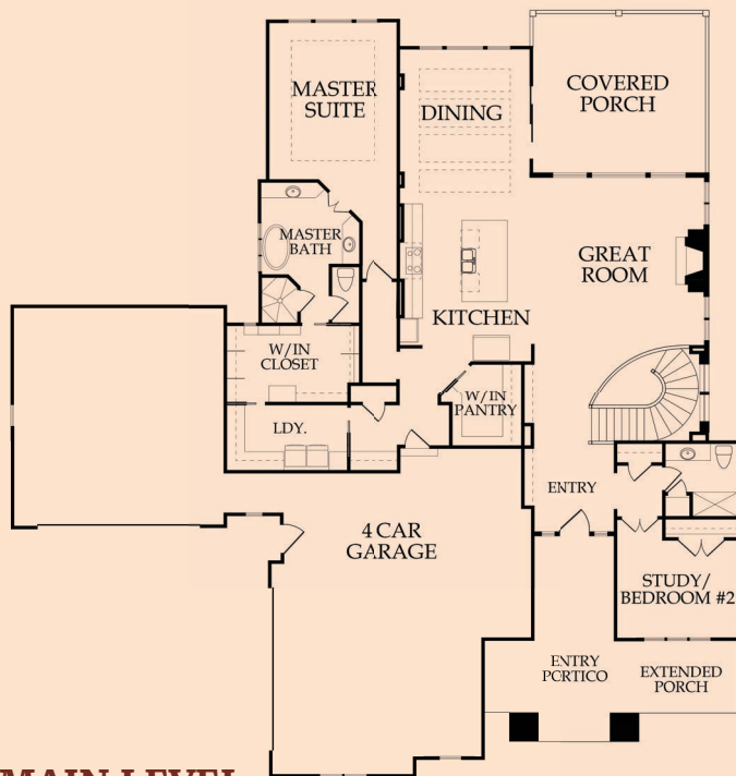
MAIN LEVEL 2,470 SQFT
