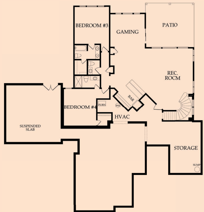
LOWER LEVEL 1,670 SQFT
