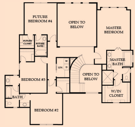
UPPER LEVEL 1,619 SQFT
