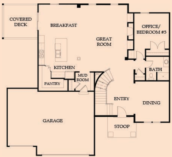
MAIN LEVEL 1,545 SQFT
